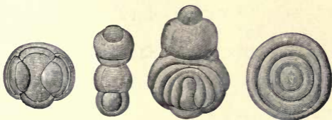
Concretions from Clay-beds.
